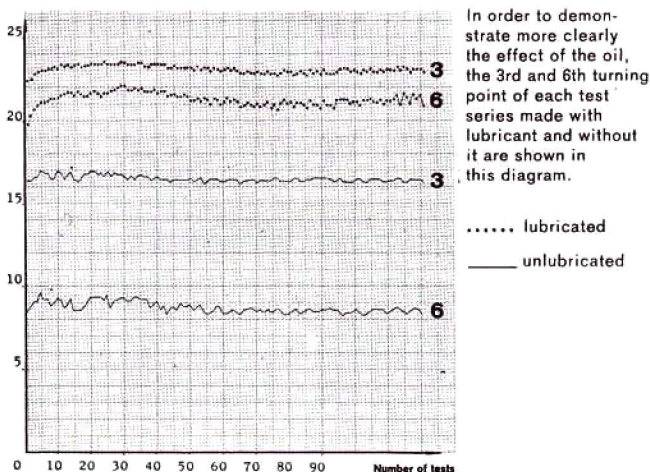
Friction pendulum diagram of prod. No. 9024: steel/Delrin 500 NC 10
