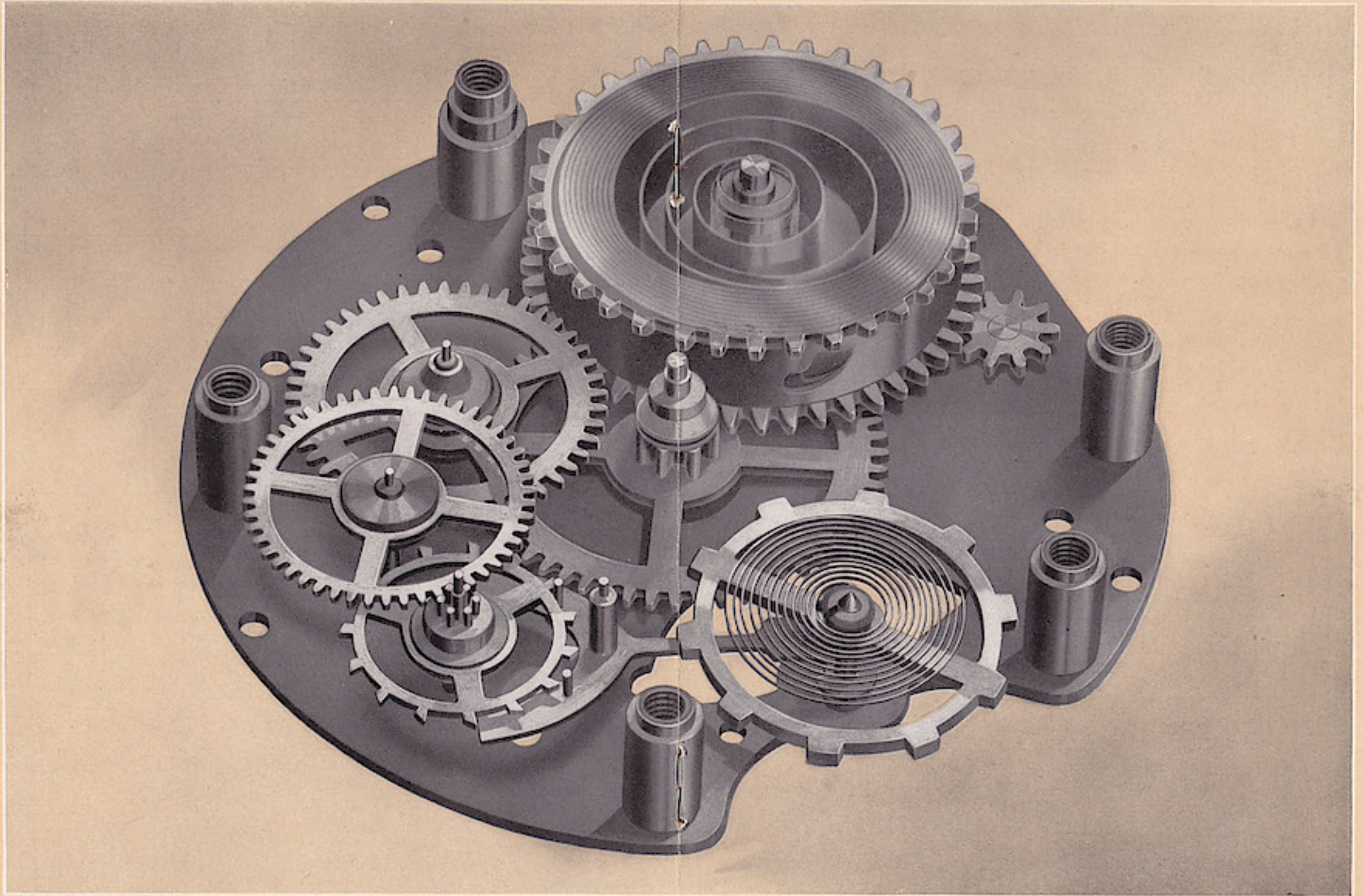
The Boyproof Watch Movement
