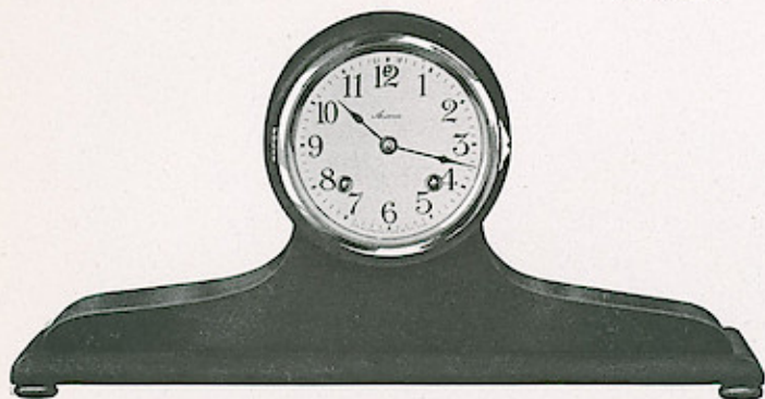
CABINET NO. 37 Height, 8¼ Inches Width, 16¼ Inches White Porcelain or Silver Dial, 4 Inches Mahogany Dull Rubbed Finish Arabic or Roman Numerals Brass Cast Sash, Dull Gold Finish White Beveled Glass 8-Day, Hour and Half-Hour Gong Strike Round Polished Pendulum Movement.
