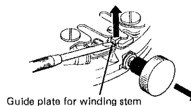
Guide plate for winding stem
